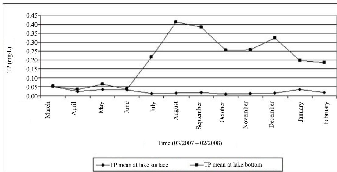
Figure 5. Mean monthly variation of TP at surface and bottom waters in Lake Amvrakia (2007-2008).
