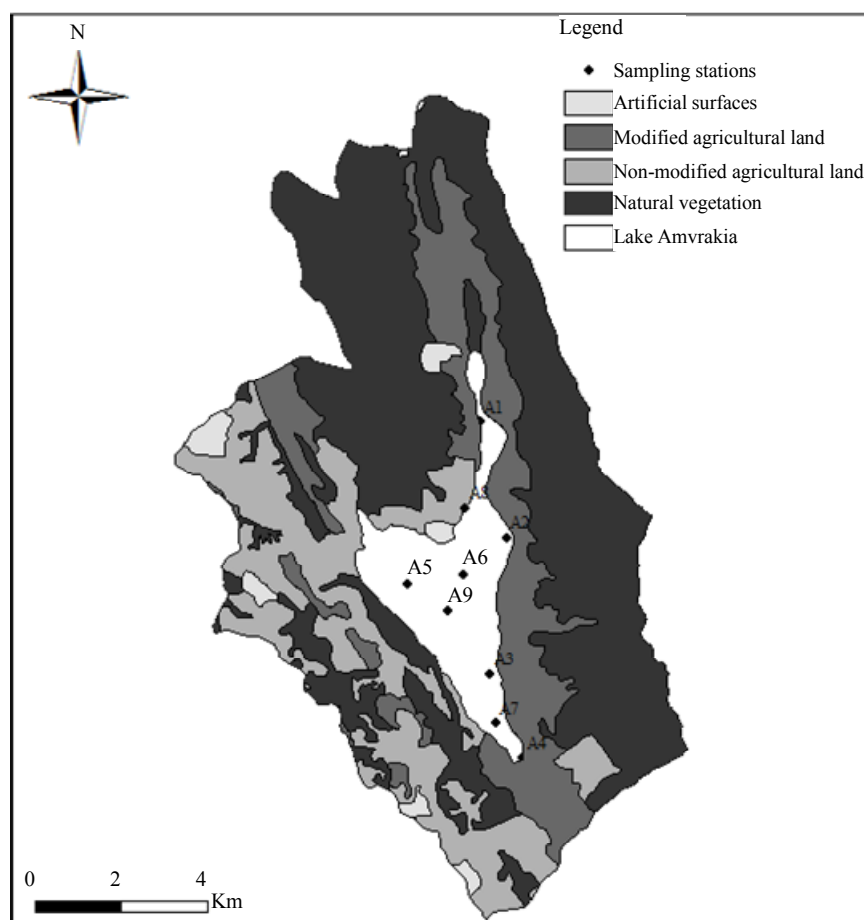
Figure 6. Map of recent land uses of Lake Amvrakia catchment. Modified agriculture, is the tobacco cultivation, which changed in the last 10 years. Non-modified is the olive trees cultivation which still exists in the area.
