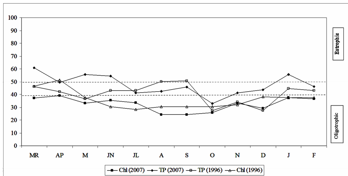
Figure 7. Monthly trophic state index of Lake Amvrakia for two periods from the station A5. (From Danielidis (1996) and our study (2007)) TP: Total phosphorus, Chl: Chlorophyll-a.
