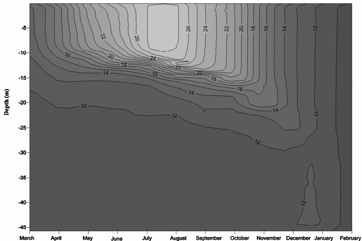
Figure 2. Monthly variation of temperature in Lake Amvrakia (2007-2008) from the station A5.
