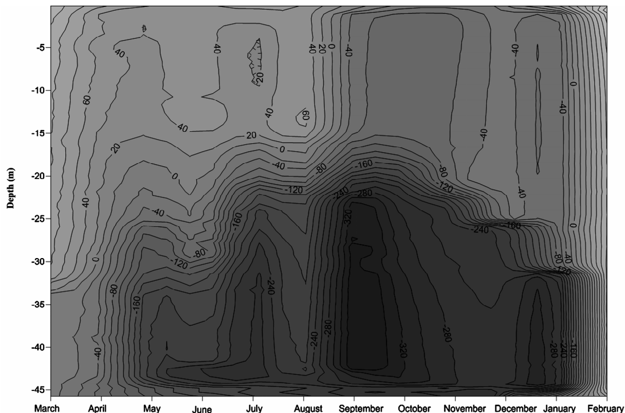
Figure 4. Monthly variation of redox potential in Lake Amvrakia (2007-2008 from the station A5).
